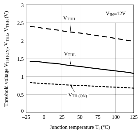
Fig.12 On Threshold Voltage vs. Junction Temperature
